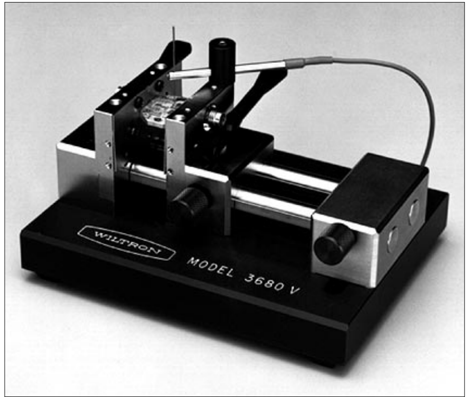
Microwave circuit provided by Fujitsu Microelectronics, Inc.
